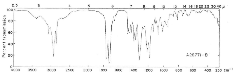
Fig. 1. Infrared spectrum of A26771B in KBr.
